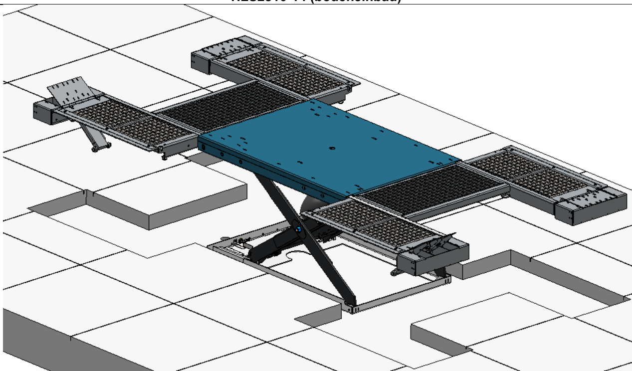
HLS2810-14 (bodeneinbau)
