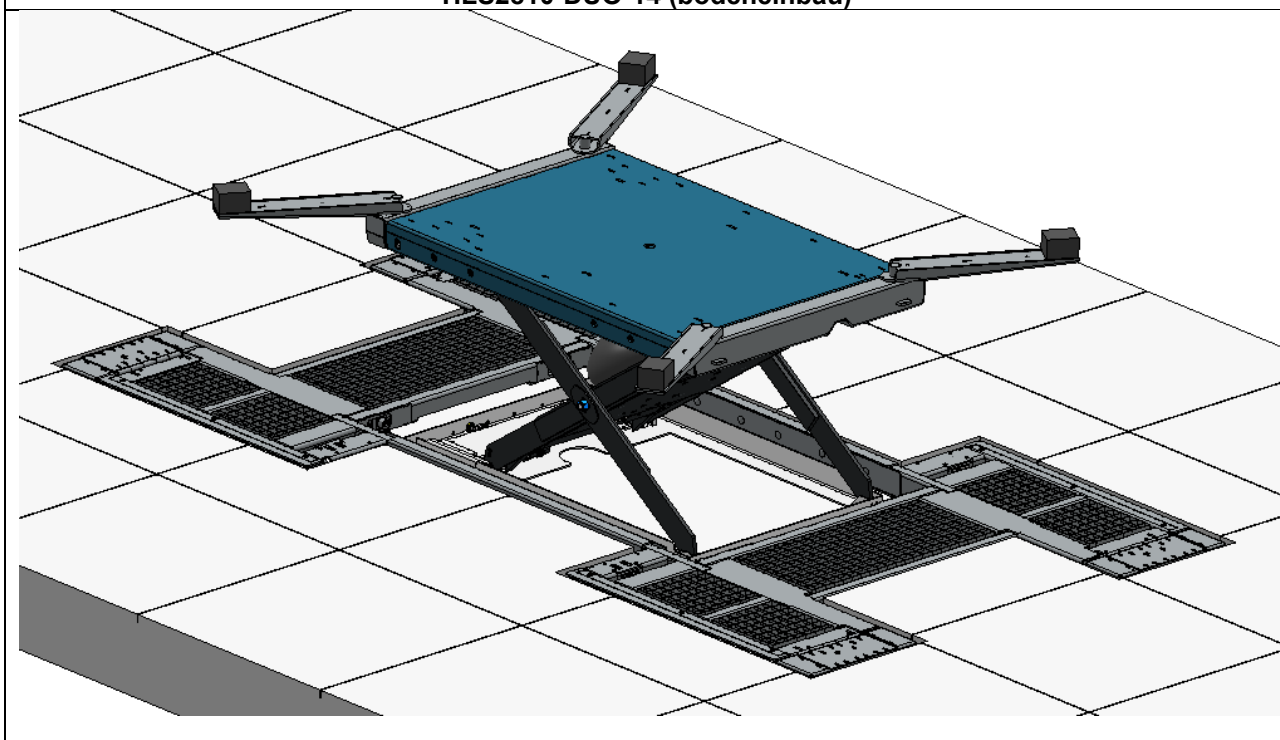
HLS2810-DUO-14 (bodeneinbau)
