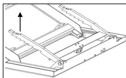
Figurer 4 / 5: Fallbrems låst fast / fallbrems hevet under senkingen
