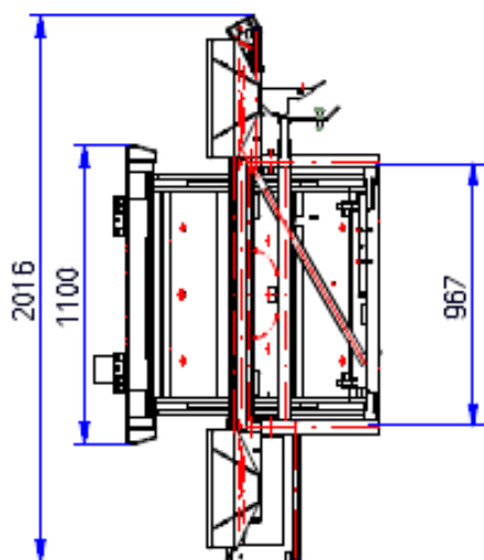
Maßblatt K1200-DUO-17 (TA1215-DUO-003-3)
